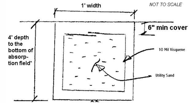
VAPOR BARRIER DETAIL
